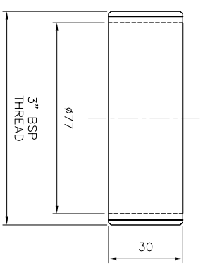
(SCALE:-1:4) DETAIL-A BUSH FOR COUPLER
